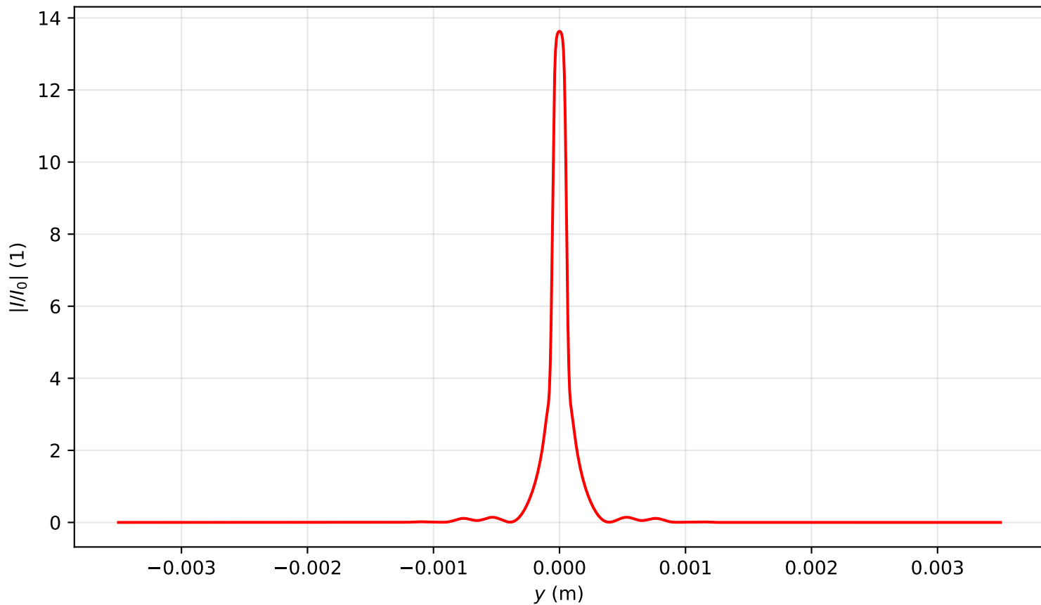
Intensity profile I(x=0, y, z=0.716)/I_0 , P_{in}=8.5P_{cr} , artificial time
